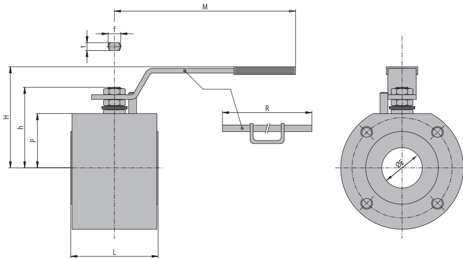
Dimensioni - outline dimensions
